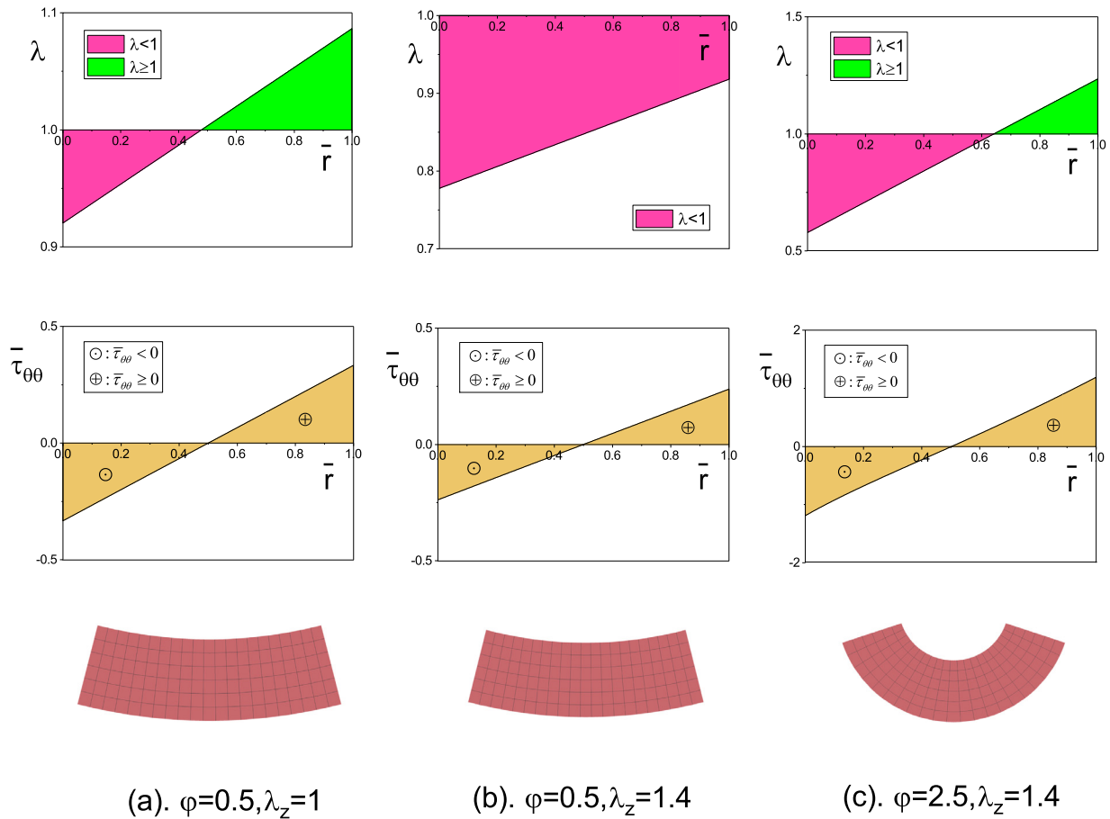
Fig. 8. Purely elastic bending of a dielectric slab which is three times wider than thick ( \bar{V}=0, A/H=3 ) for various bending angles and axial elongation ratios: (a) \bar{\varphi}=0.5, \lambda_z=1 ; (b) \bar{\varphi}=0.5, \lambda_z=1.4 ; (c) \bar{\varphi}=2.5, \lambda_z=1.4 . The top, middle and bottom rows show the variations through the thickness of the circumferential stretch and of the stress distributions, and the resulting bending shapes, respectively.
