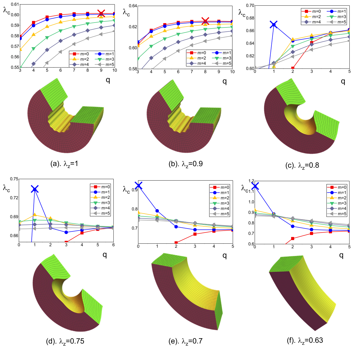
Fig. 14. Bending instability of dielectric slabs with A/H = 3, L/H = 1.5, \bar{V} = 0.3 and subject to (a) \lambda_z = 1 ; (b) \lambda_z = 0.9 ; (c) \lambda_z = 0.8 ; (d) \lambda_z = 0.75 ; (e) \lambda_z = 0.7 ; (f) \lambda_z = 0.63 . The top rows are plots of \lambda_c versus q for a range of modes m = 0 - 5 and bottom rows are the corresponding wrinkling shapes when instability occurs. In cases (a) and (b), circumferential wrinkles occurs and in cases (e) and (f), axial wrinkles occurs whereas in cases (c) and (d), a two dimensional (circumferential and axial) pattern emerges.
