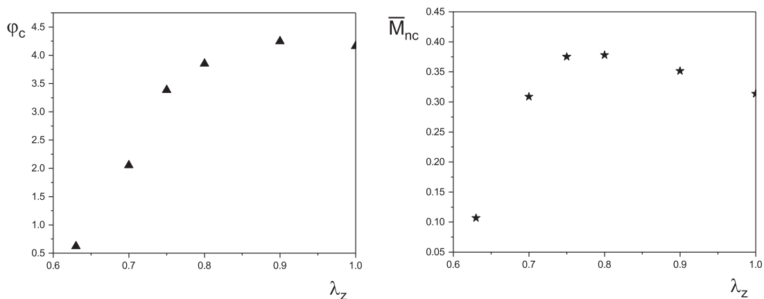
Fig. 15. Effect of the axial compression, as measured by the axial stretch ratio \lambda_z , on the critical values of bending angle \varphi_c and moment \bar{M}_{nc} for dielectric slabs with A/H = 3, L/H = 1.5, \bar{V} = 0.3 .
