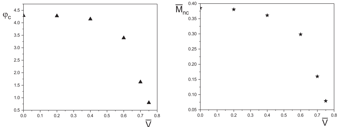
Fig. 13. Effect of the applied voltage \bar{V} on the critical values of bending angle \varphi_c and moment \bar{M}_{nc} for dielectric slabs with A/H = 3, L/H = 1.5, \lambda_z = 0.85 .
