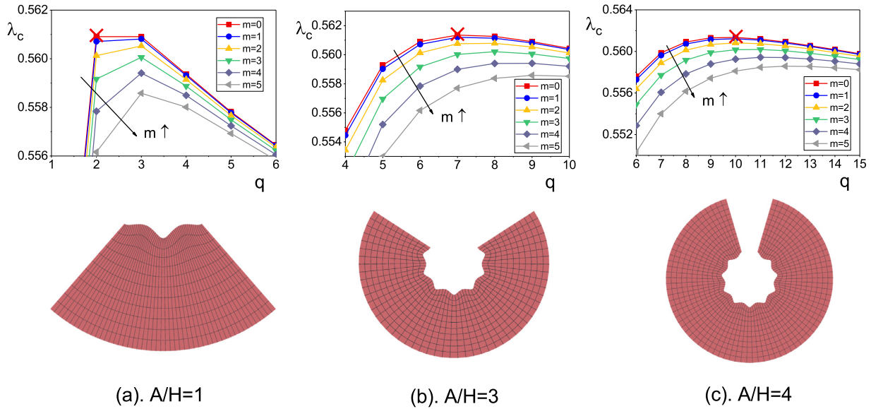
Fig. 10. Elastic bending instability of a dielectric slab with fixed axial compression ( \bar{V} = 0, \lambda_z = 1 ) for various width aspect ratios: (a) A/H = 1 ; (b) A/H = 3 ; (c) A/H = 4 and fixed length aspect ratio L/H = 10 . The top row shows plots of the critical circumferential stretch \lambda_c versus the number of circumferential wrinkles q for a range of axial modes m = 0 - 5 . The bottom row shows the corresponding wrinkling shapes when instability occurs. The highest point of \lambda_c - q curves for each case is marked by cross, representing the onset of the instability. In this case the m = 0 plot is always on top and there are no axial wrinkles, only circumferential.
