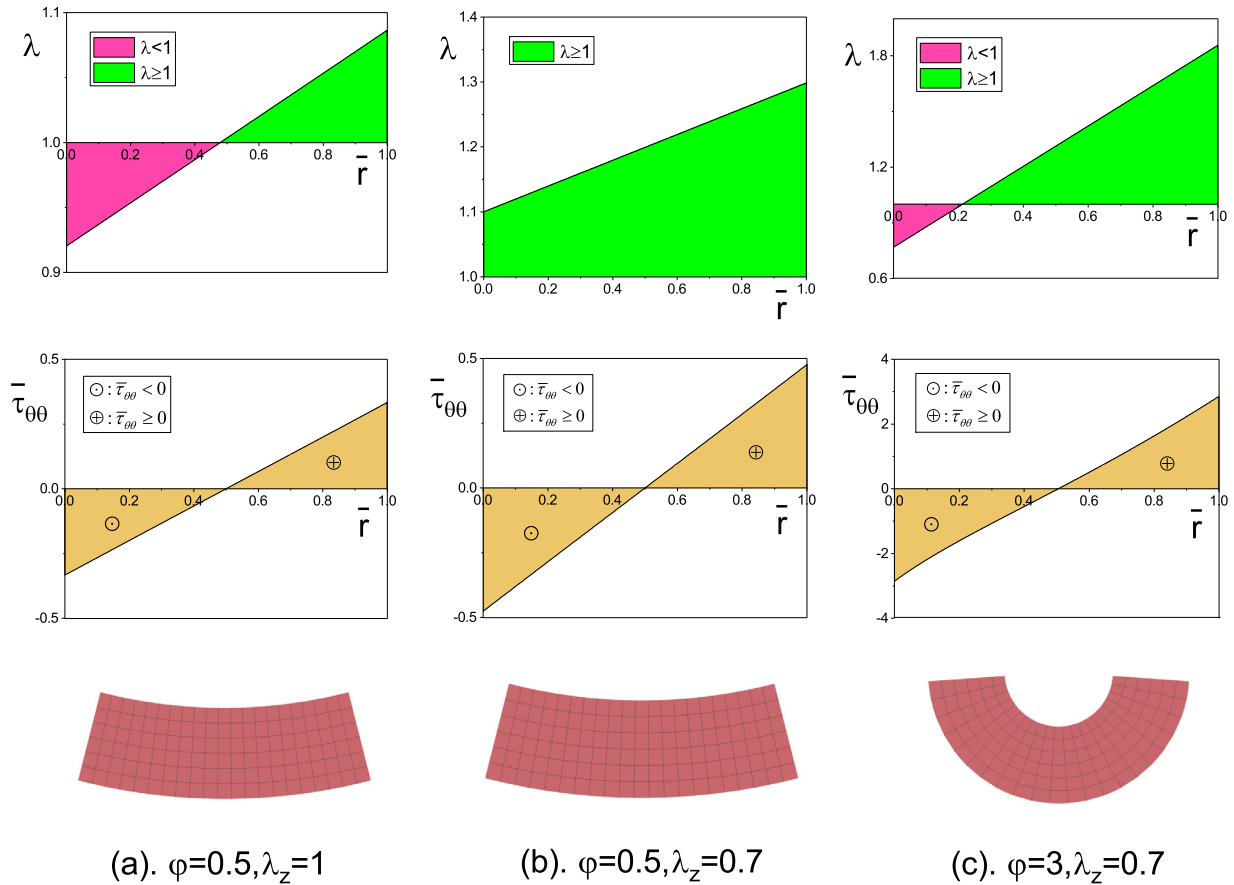
Fig. 7. Purely elastic bending of a dielectric slab which is three times wider than thick ( \bar{V} = 0, A/H = 3 ) for various bending angles and axial compression ratios: (a) \varphi = 0.5, \lambda_z = 1 ; (b) \varphi = 0.5, \lambda_z = 0.7 ; (c) \varphi = 3, \lambda_z = 0.7 . The top, middle and bottom rows show the variations through the thickness of the circumferential stretch and of the stress distributions, and the resulting bending shapes, respectively.
